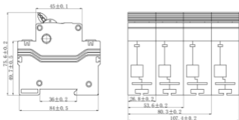
Fig.1 overall and mounting dimensions
