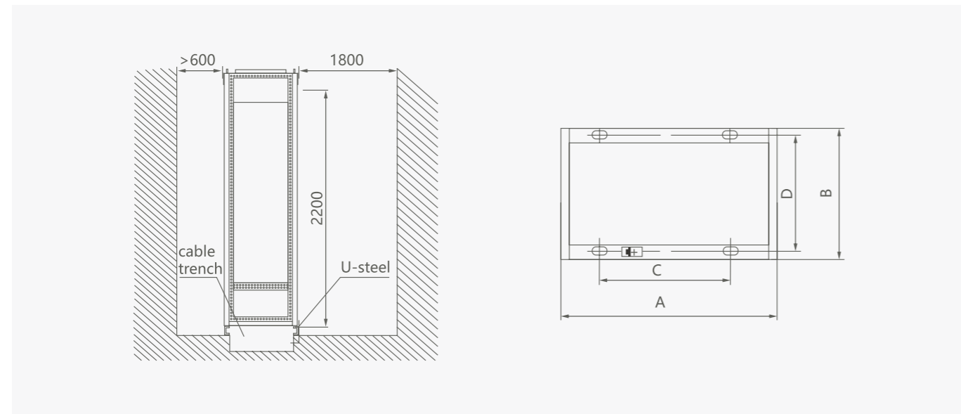
Installation Overall and mounting dimensions(mm)
