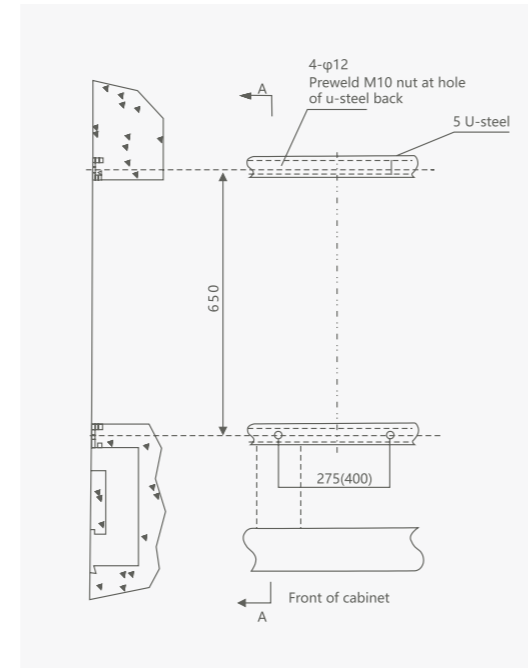
Cable incoming and outgoing configuration
