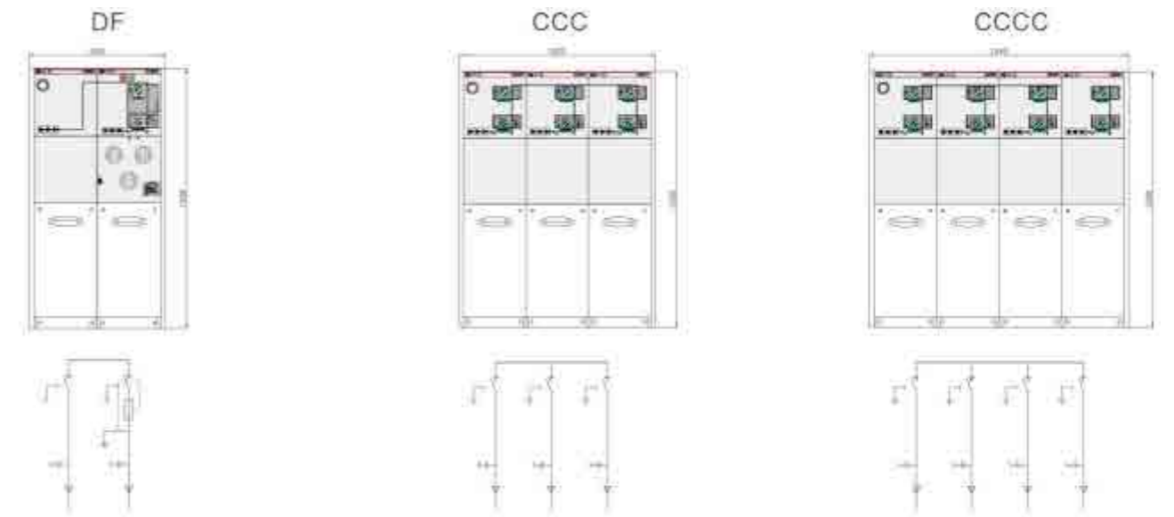
Standard 2 circuits DF (260kg)
