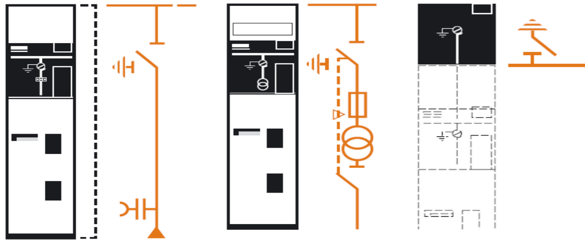
Disconnector unit (375/500 mm)
