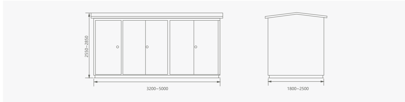
Type 1 layout
