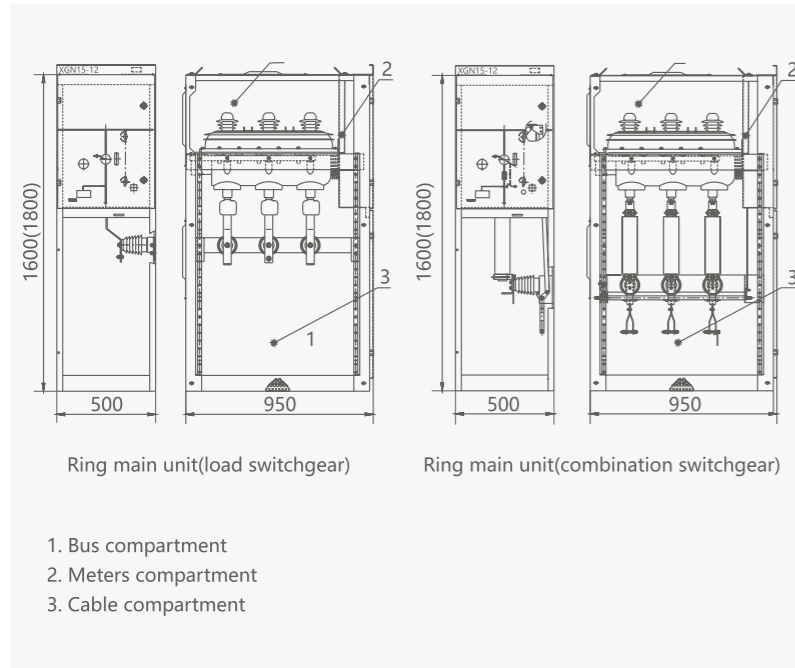
Switchgear installation Overall and mounting dimensions(mm)
