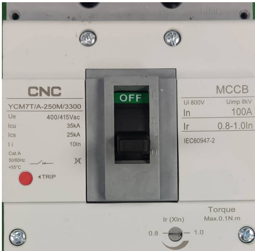
YCM7T/A-250M/3300, 3P 100 A
