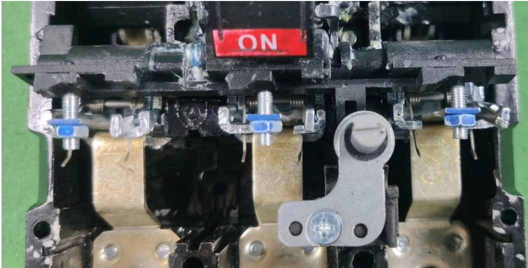
View of thermal bimetal components and leading lever, 55 °C YCM7T/A-250M/3300, 3P 100 A
