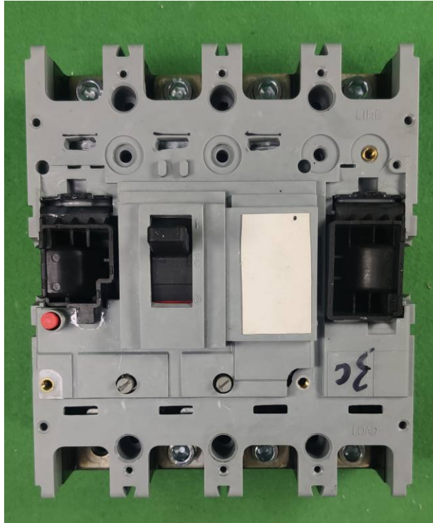
Internal view without front cover, YCM7RT-250M/4300, 4P, 250 A
