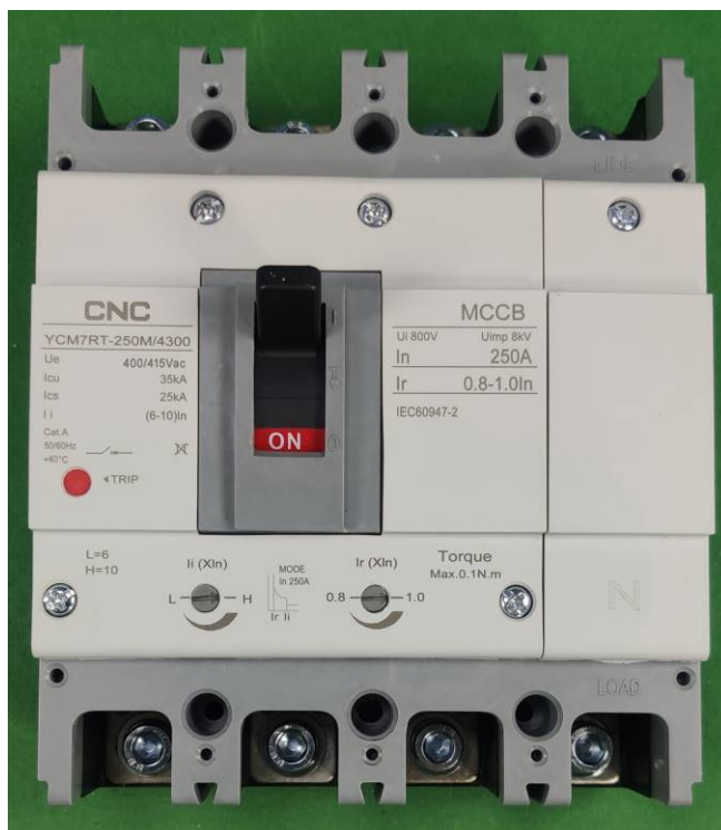
Front view, YCM7RT-250M/4300, 4P, 250 A
