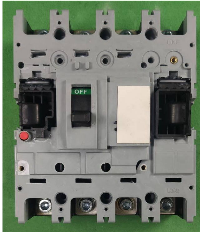
Internal view without cover, YCM7-250M/4300, 4P 250 A
