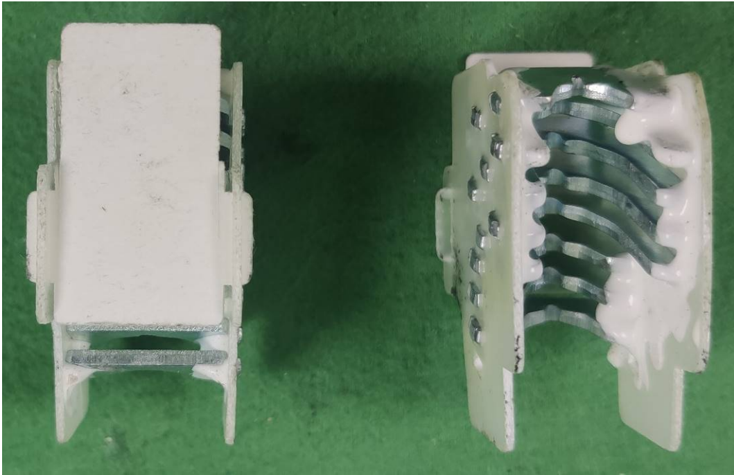
Arc chamber
