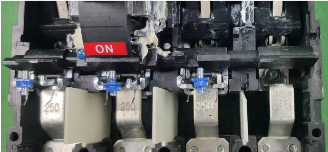
View of thermal bimetal components and leading lever, 40 °C YCM7-250M/4300, 4P 250 A
