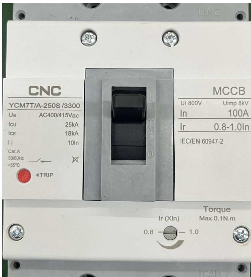
YCM7T/A-250S/3300, 3P 100 A
