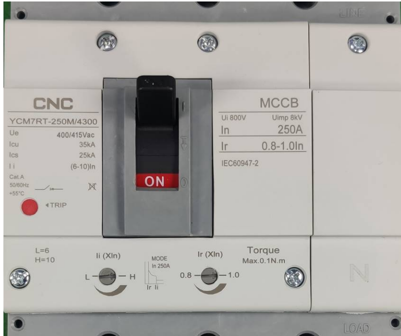
YCM7RT-250M/4300, 4P, 250 A
