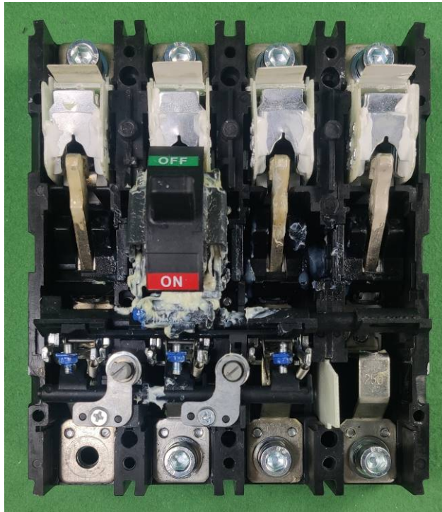
Internal view, YCM7RT-250M/4300, 4P, 250 A
